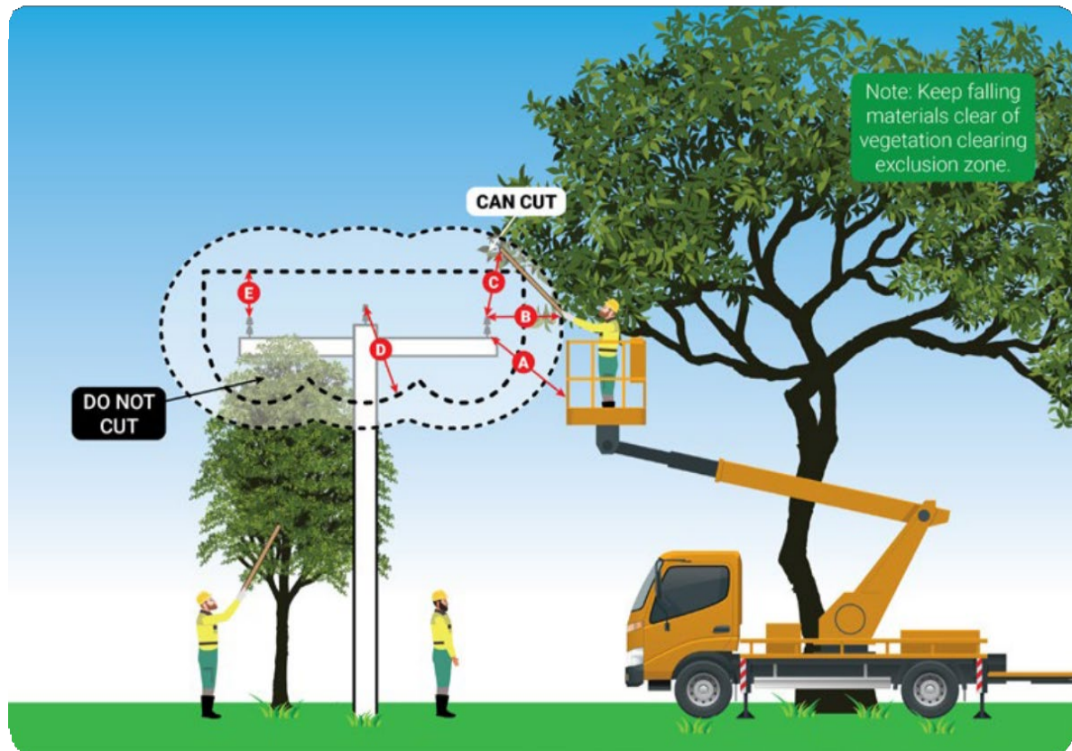
Figure 5: Safe approach distances and vegetation clearances utilising insulated mobile plant, tools and equipment (refer to Table 5).
