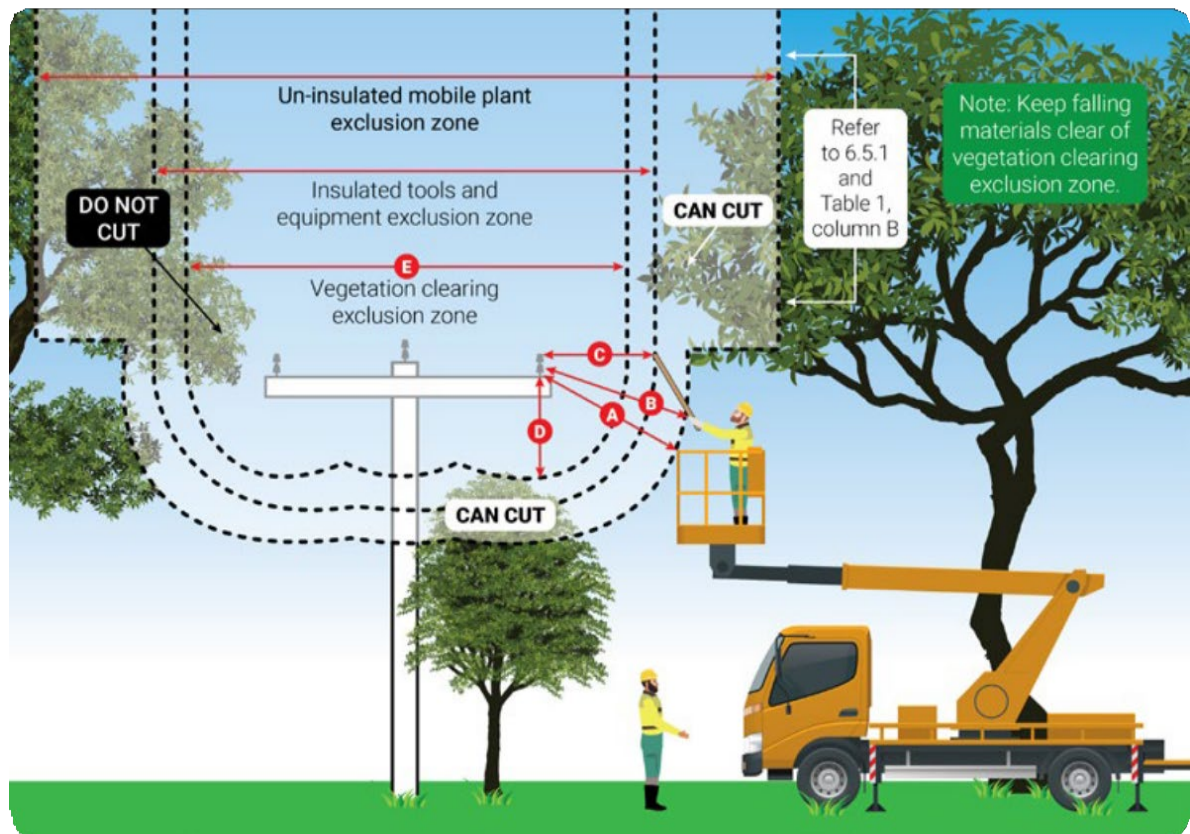
Figure 4: Safe approach distances and vegetation clearances utilising Un-insulated mobile plant, insulated tools and equipment (refer to Table 4).
