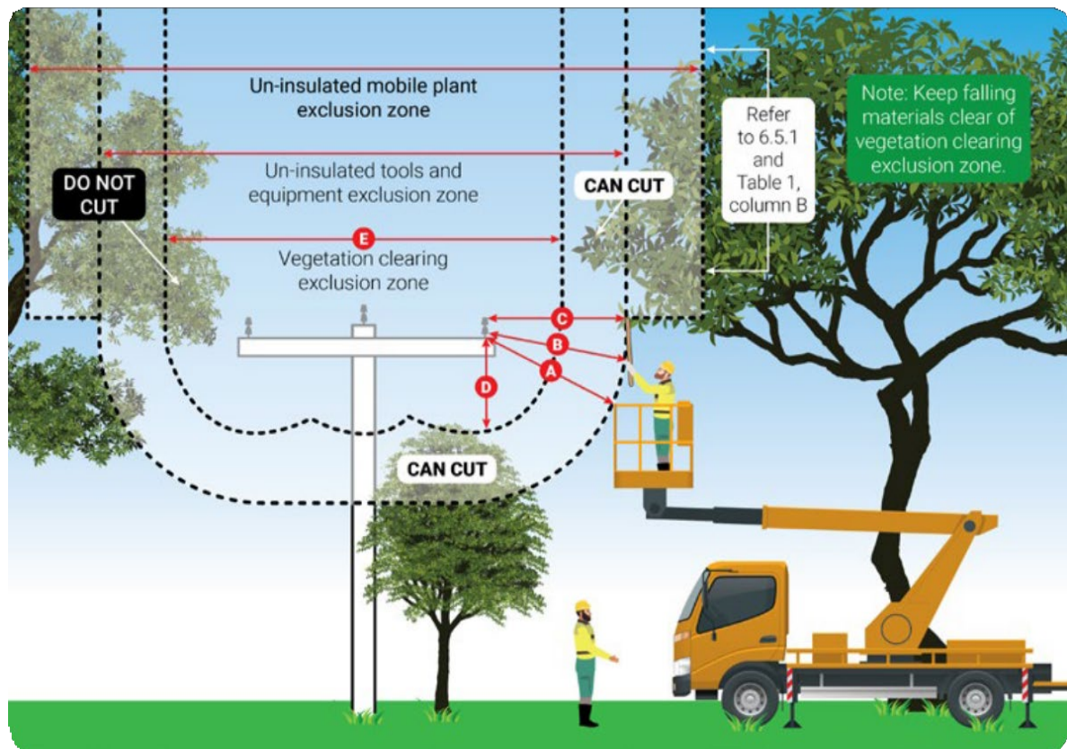
Figure 3: Safe approach distances and vegetation clearances utilising Un-insulated mobile plant, tools and equipment (refer to Table 3).
