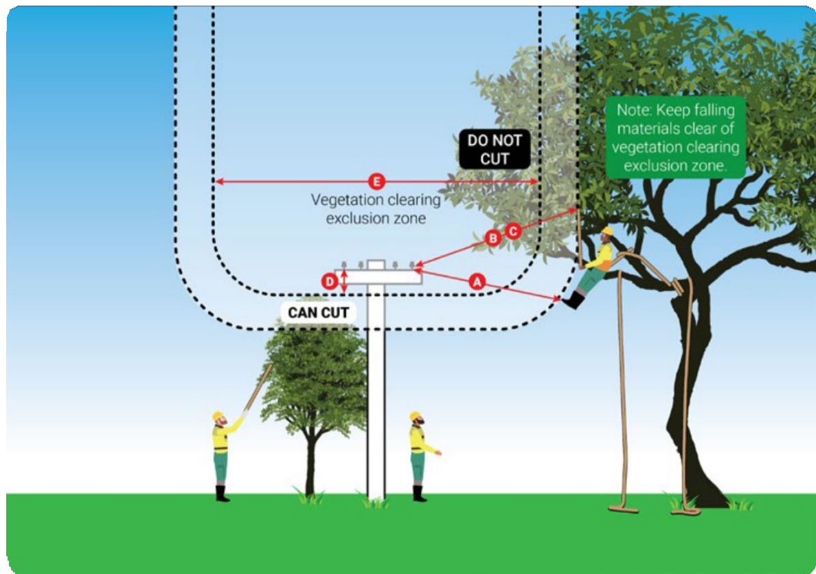
Figure 2: Safe approach distances for climbing vegetation workers (Refer Table 2).
