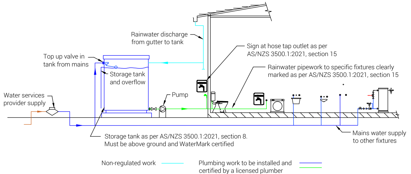
Diagram 3 – Water supply plumbing installation from a storage tank with mains and rainwater top up to plumbing fixtures approved for use with rainwater.
