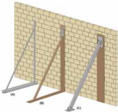
Figure 5: Examples of typical types of temporary supports (not to scale)
